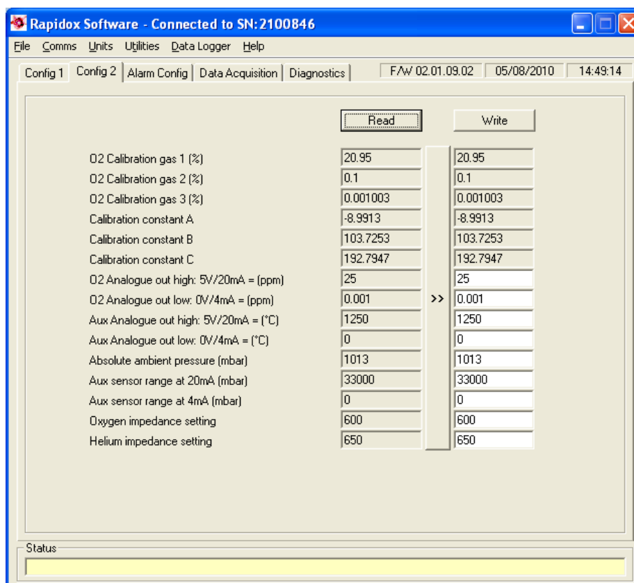
Figure 12: Configuration 2 screen. Note the actual values used may differ from those shown above.
