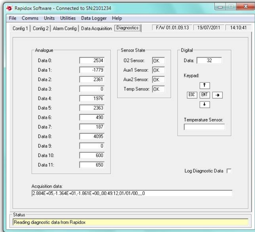
Figure 23: Rapidox Diagnostics Page
